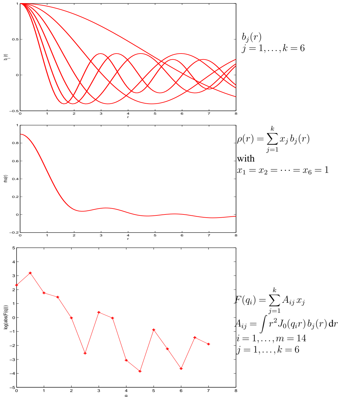
Fig. 1: a) basis functions b_j(r) , b) \rho(r) , c) data F(q_i) in a logarithmic scale.
